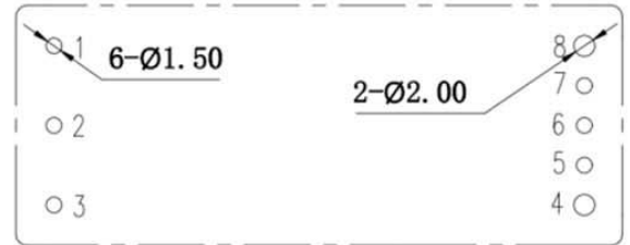
Recommended PCB slot dimension
